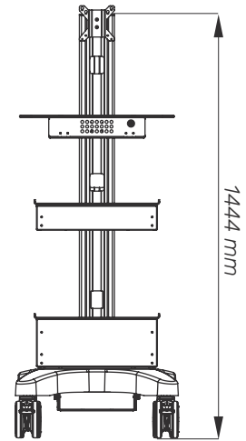
Side
