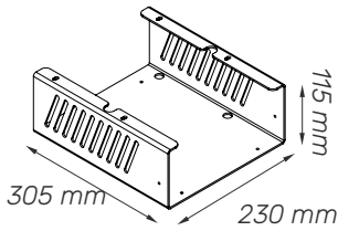
Transformer holder
