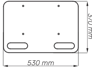
Work surface
