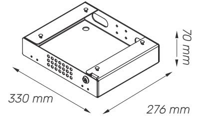
Computer holder
