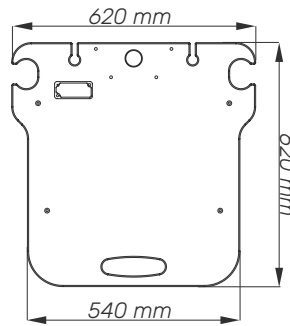
Worksurface
