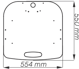
Worksurface
