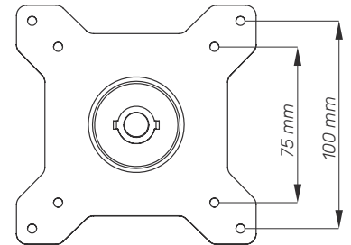
VESA Mount up to 24"
