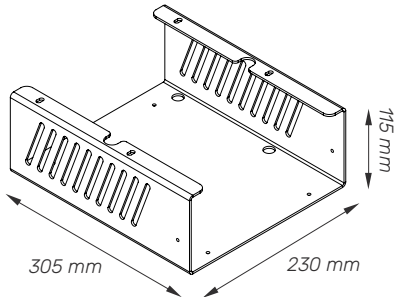
Isolation transformer holder
